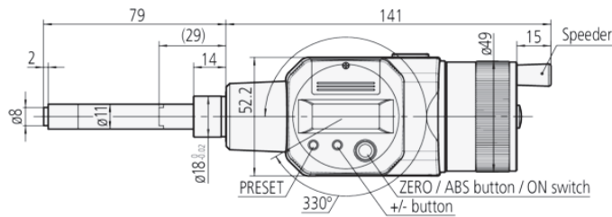
Digital Micrometer, Order No. 00-99-901-4889
